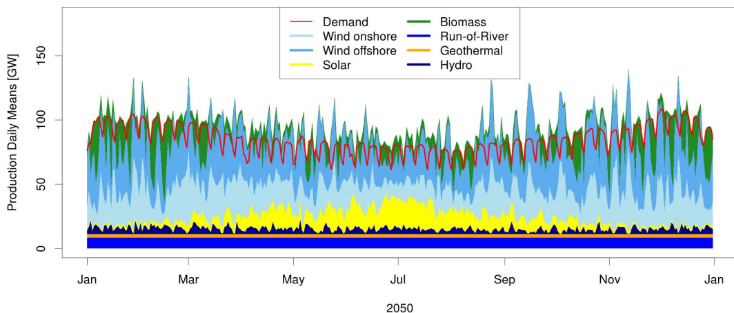
FIGURE 5.11: Example Application: One possible compilation of demand and renewable electricity production in the course of the year 2050 summarized for the whole Baltic Sea region. Source: CSES (2012, p.15, Figure 10)
