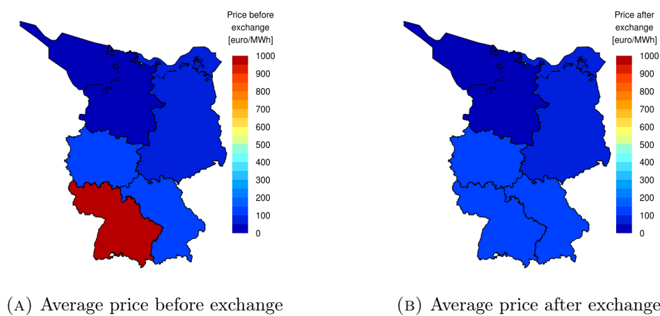
FIGURE 5.9: renpass plot output example: Average prices of test scenario 5. Comparison of prices before and after electricity exchange shows that they converge: The lack of electricity indicated by a high price in southwestern Germany (red) can be countered by importing which lowers the average price in that region. Source: own image of renpass
