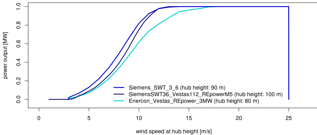
FIGURE 4.7: Performance curves of wind power plants stored in the renpass database, normalized to a rated power of 1 MW. For wind onshore, the joint 3 MW (turquoise) and for offshore, the joint 5 MW (dark blue) performance curve is utilized. Source: illustration based on Bons (2014)
