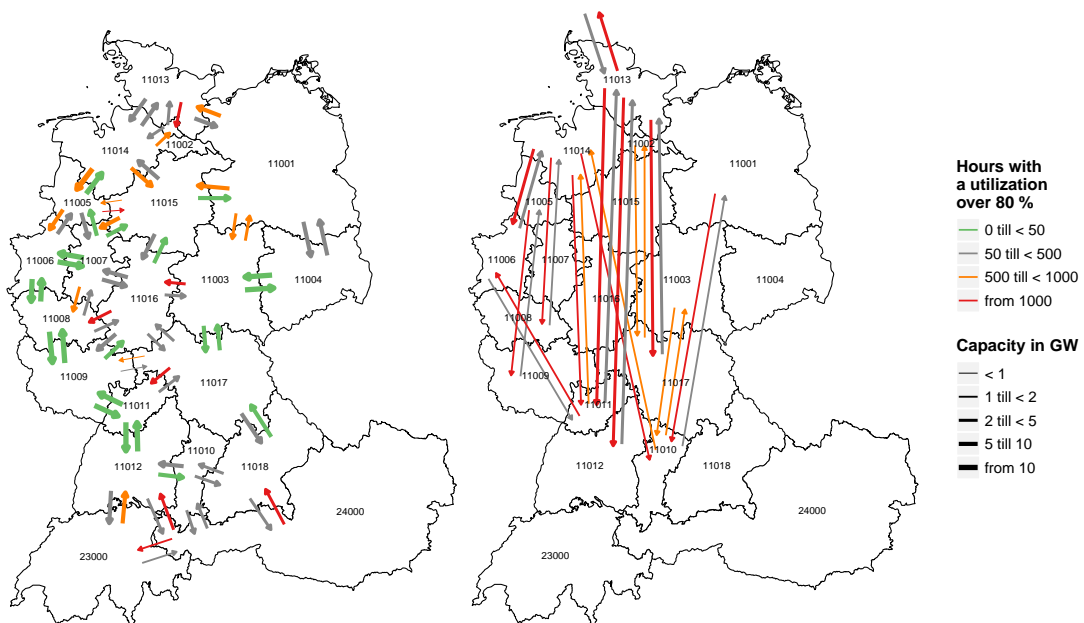
FIGURE 5.14: Usage rate of the transmission lines HVAC (left) and HVDC (right) in the year 2032. Scenario C with wind power capacity shifted to the south of Germany. Source: (Bons, 2014, p.89, Figure 5.6(b))
