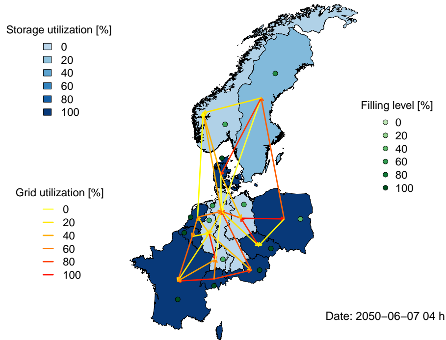
FIGURE 5.16: Storage utilization, grid utilization and filling level in the modeled countries in scenario 16003 during the hour of maximal excess electricity. The storage capacities of countries without pumps are considered as 100% utilized and their reservoirs filled to 100%. Source: Böhm (2014, Figure 2, p.3)
