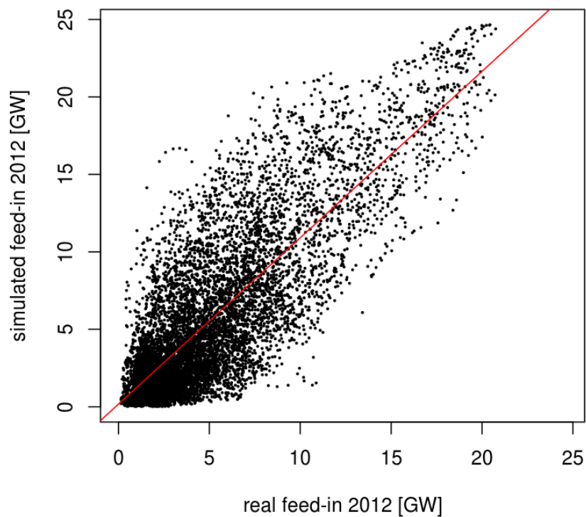
FIGURE 4.8: Calibration of onshore wind power curve in renpass compared to real and simulated feed-in. Regression line in red. Source: own image
