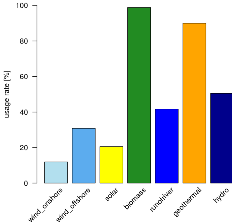
FIGURE 5.6: Example of plot output: Usage rates of utilized energy sources for the whole simulation area in July - Test scenario 7. Source: own image of renpass.
