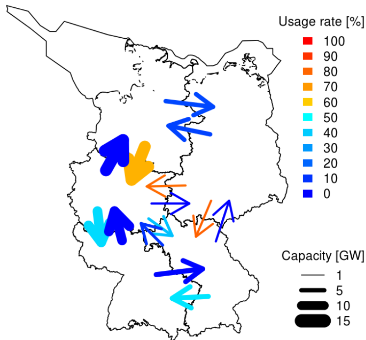
FIGURE 5.10: renpass plot output example: The colors of the arrows reflect the usage rate [% of grid capacity in the simulation time] and the capacity of the connections [GW] is illustrated by the width of the arrows (Test scenario 5). Source: own image of renpass
