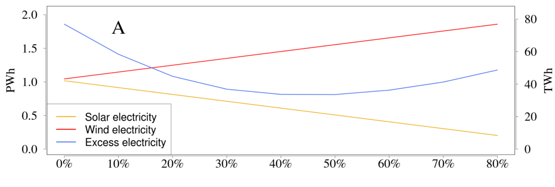
FIGURE 5.15: Excess electricity subject to the proportion of onshore wind and solar. Source: Söthe (2014, Figure 2, p.3)
