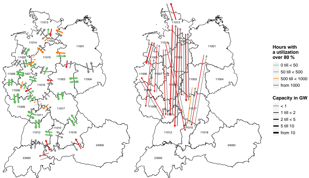
FIGURE 5.13: Usage rate of the transmission lines HVAC (left) and HVDC (right) in 2032. Scenario A in this study is based on scenario assumptions of Grid Development Plan Scenario B. Source: (Bons, 2014, p.81, Figure 5.2)
