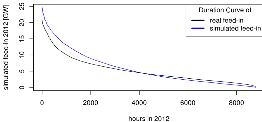
FIGURE 4.9: Calibration of onshore wind power curve in renpass compared to real and simulated feed-in: duration curve. Source: own image
