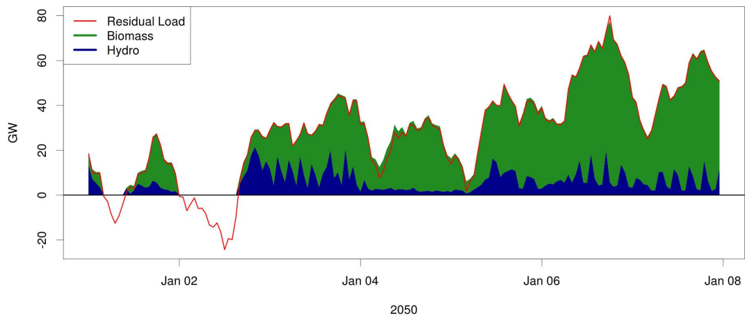
FIGURE 5.12: Example Application: Hydro and biomass electricity feed-in covering the residual load in the Baltic Sea region in January 2050. Source: CSES (2012, p.17, Figure 12)
