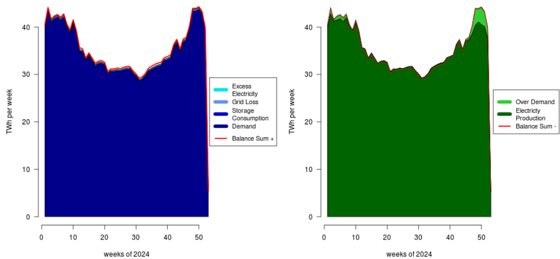
(A) Weekly sums of demand, storage consumption, grid losses and excess electricity (B) Weekly sums of electricity production and excess demand
