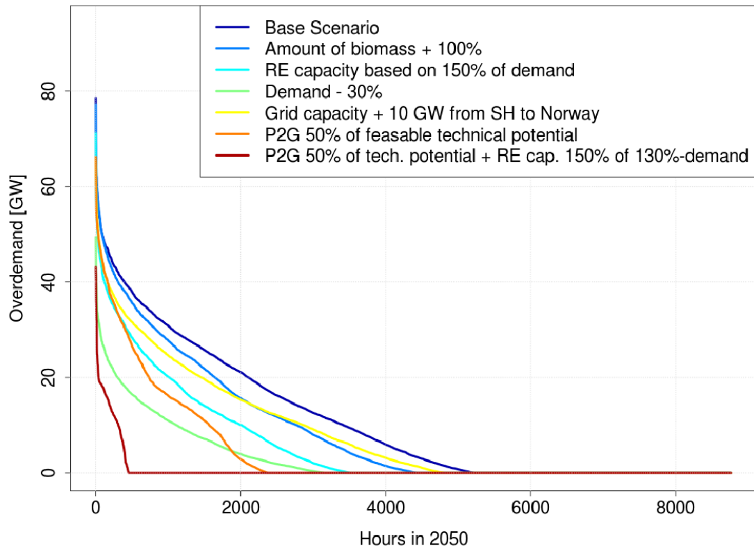
FIGURE 5.18: Parameter influence on the excess demand duration curve in Germany. Source: Kaldemeyer (2014, Figure 3.1, p.3)
